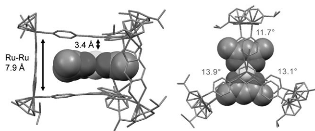
Figure 1. Molecular structure of [(acac)_2PtC1]^{6+} ; side view and top view.
