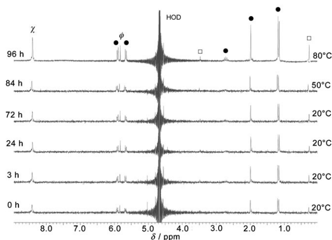
Figure 2. 1 H NMR spectra of [(acac)_2PdC1]^{6+} (D 2 O, 200 MHz) at elevated temperature (□ acac, ϕ dhbq, χ tpt, ● p -PrC 6 H 4 Me).
