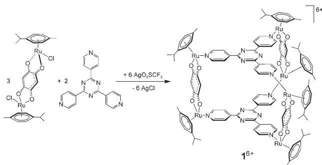
Scheme 1. Synthesis of 1 ( \text{O}_3\text{SCF}_3 ) 6 .
